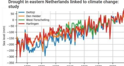
Sea level measured in Dutch coastal stations
